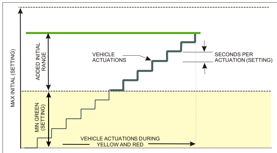
VARIABLE INITIAL INTERVAL TIMING DETERMINATION VARIABLE INITIAL BETWEEN MIN. GREEN AND MAX. INITIAL
