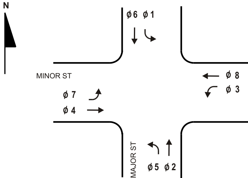
NORTH-SOUTH AS MAJOR STREET FOR 8-PHASE CONTROLLER
