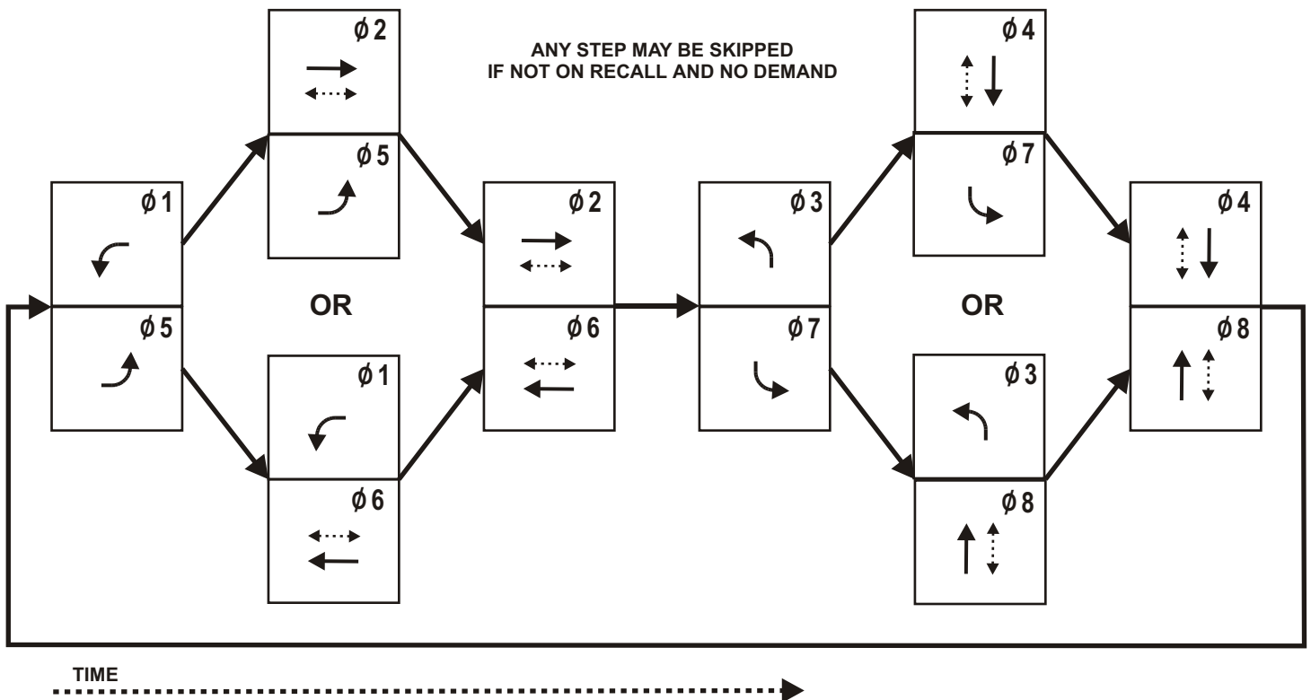
NEMA 8-PHASE ACTUATED CONTROLLER PHASING SEQUENCING
