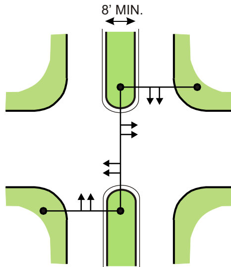
Z-SPAN (WITH CURBED MEDIAN)
