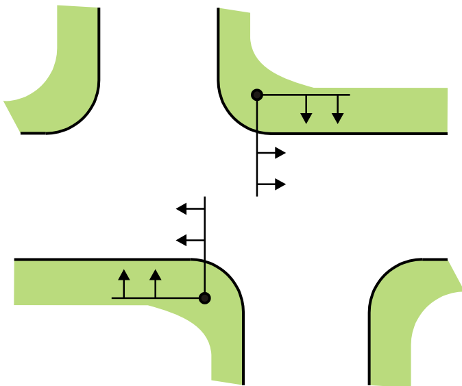
DUAL MAST ARMS (OFFSET INTERSECTION)
