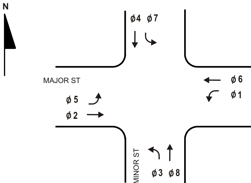
EAST-WEST AS MAJOR STREET FOR 8-PHASE CONTROLLER
