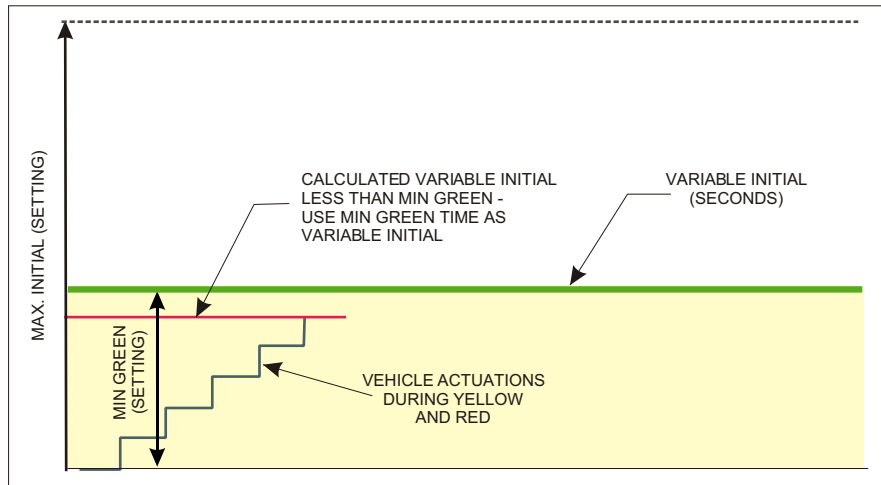
VARIABLE INITIAL INTERVAL TIMING DETERMINATION CALCULATED VARIABLE INITIAL LESS THAN MIN. GREEN
