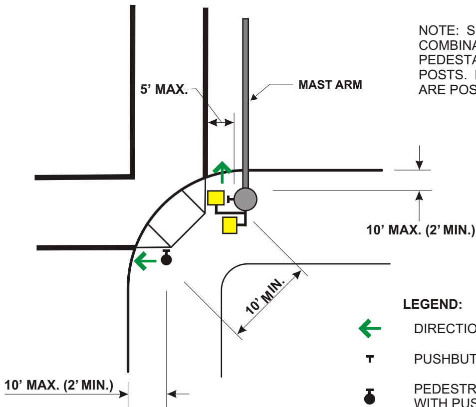
CORNER WITH SINGLE RAMP
