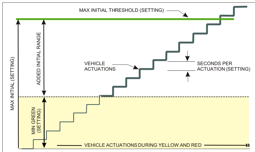
VARIABLE INITIAL INTERVAL TIMING DETERMINATION CALCULATED VARIABLE INITIAL GREATER THAN MAX. INITIAL
